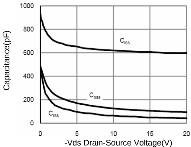
Figure 5. Capacitance
